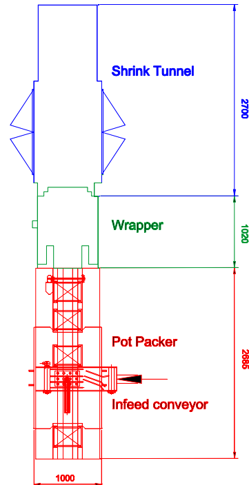
Typical installation shown with Ancram Shrink Wrap and Shrink Tunnel
