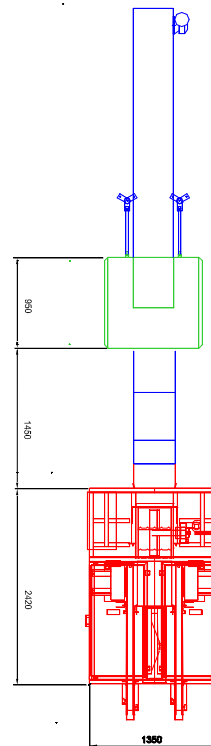
Footprint of in-line Crate Packer and Stacker
